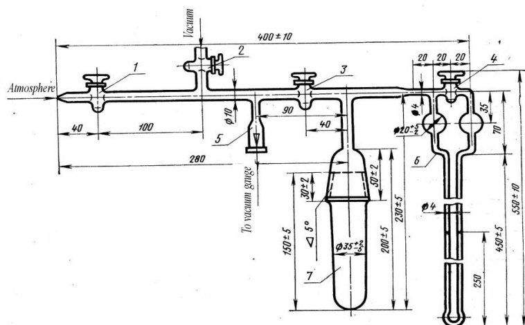
Fig. 3.4.3.6.1 Measuring device for determination of diffusible hydrogen content (GOST 23338-91, method 2): 1, 2, 3, 4 — vacuum cocks; 5 — vacuum-gauge lamp; 6 — oil pressure gauge; 7 — gas burette
